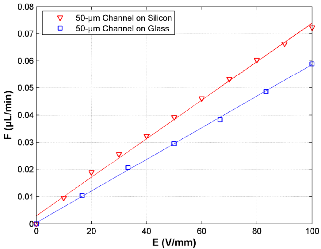
Figure 2.6. Expanded view of the flow rates generated in single 50-µm channel EOF pumps.
