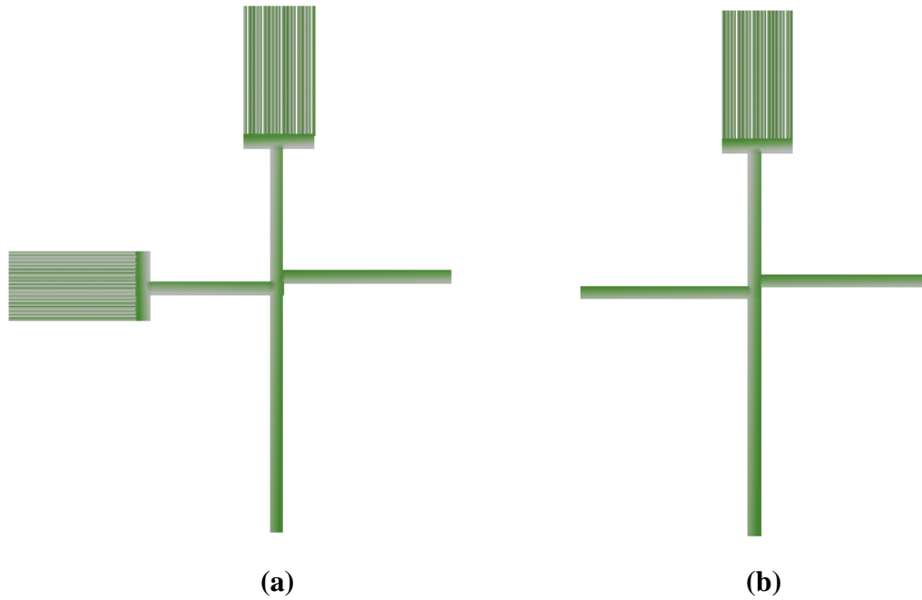
Figure 4.1 Microfluidic channel designs for surface modification experiments using (a) two EOF pumps and (b) a single EOF pump.
